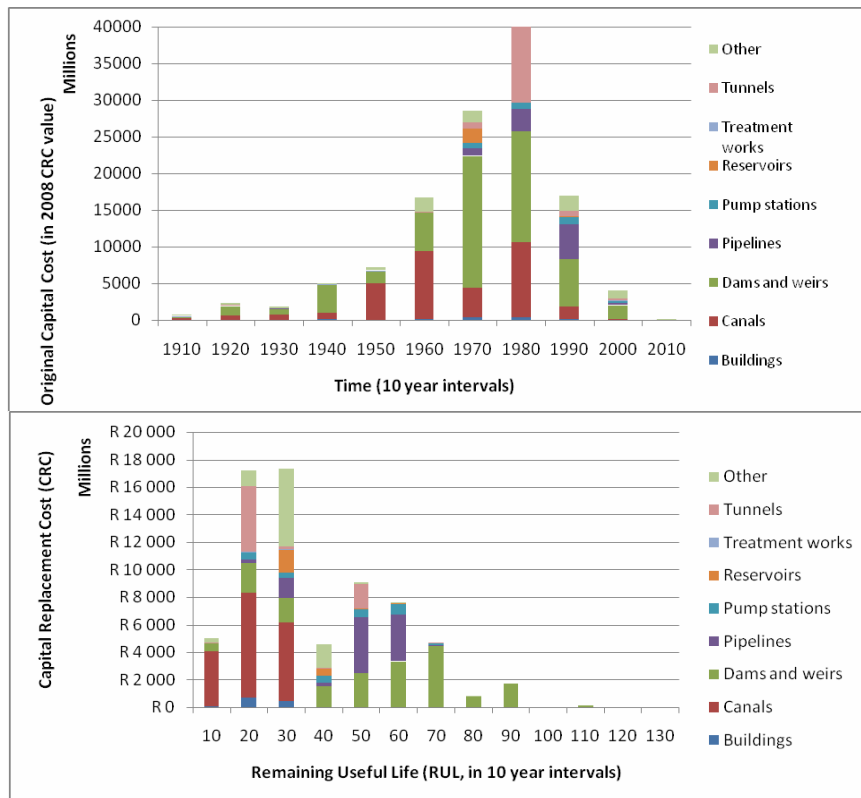
Figure 3. The age profile of assets currently on the books of the Department of Water Affairs and Forestry (DWAf) shows a peak period of capital investment in the 1980’s followed by a dramatic decline (top). The remaining useful life of those assets shows a worrying trend (bottom). Both of these graphs have a similar pattern to Figure 1 suggesting a trend towards the erosion of the assurance of supply needed to grow the national economy in a sustainable manner. (Both graphs courtesy of DWAf, 2008).
